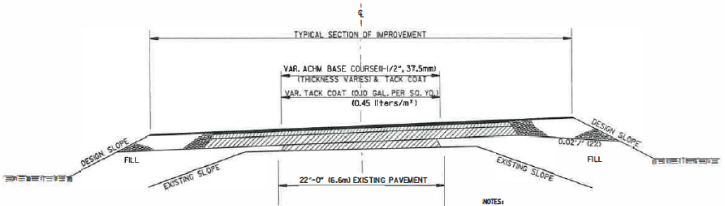
METHOD OF RAISING GRADE
